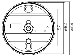
ceiling base dimensions
